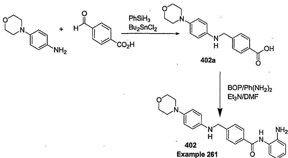
Scheme 59
